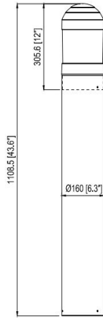
42" BRB
